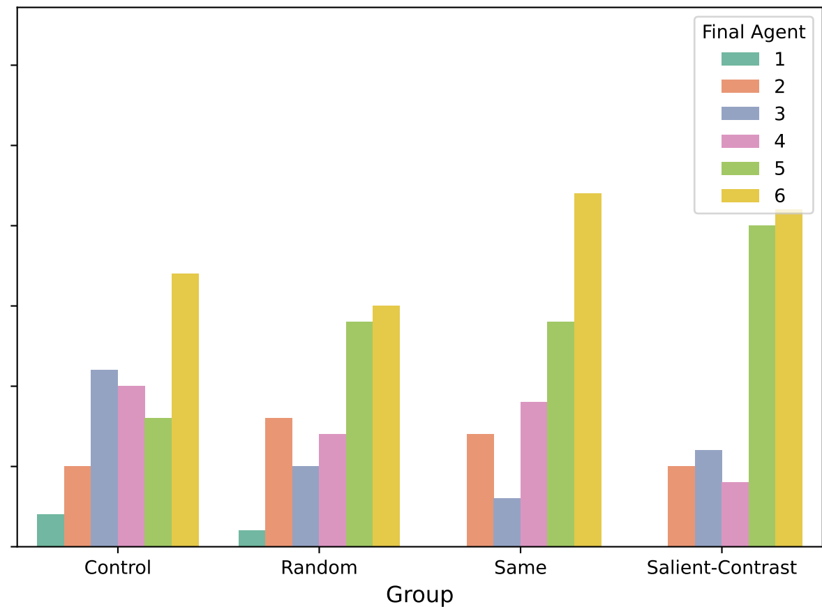
FruitBot
